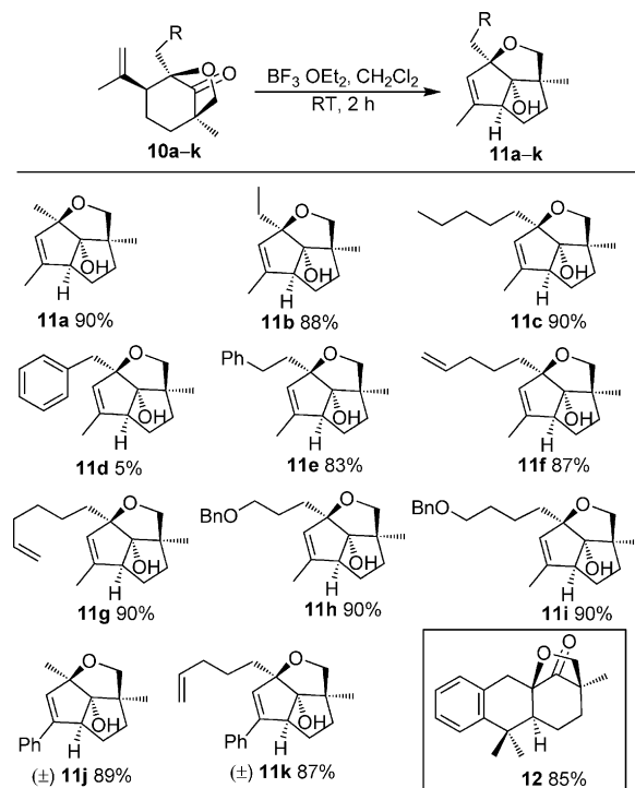
Scheme 4. \text{BF}_3\cdot\text{Et}_2\text{O} -mediated rearrangement of substituted 6-oxabicyclo[3.2.1]octan-8-ones 10a–k to the 2,8-oxymethano-bridged diquinanes 11a–k .
